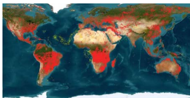
Figure 3.1 Active fires detected by MODIS worldwide in July 2022. Adapted from NASA
